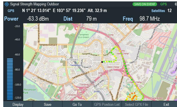
Identifying the area of interest with the R&S®FPH-K16
