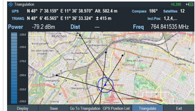
Triangulating the interferer location with the R&S®FPH-K15
