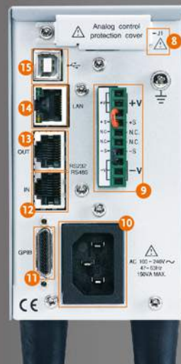
PFR-100M后面板
