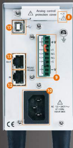
PFR-100L后面板
